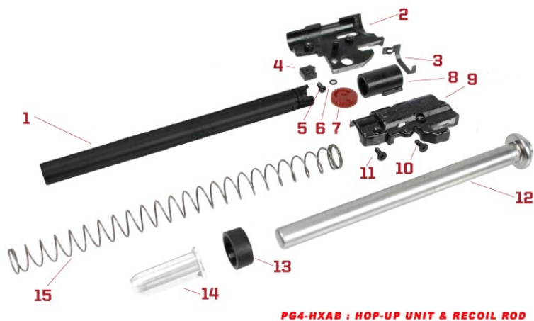
PG4-HXAB : HOP-UP UNIT & RECOIL ROD
